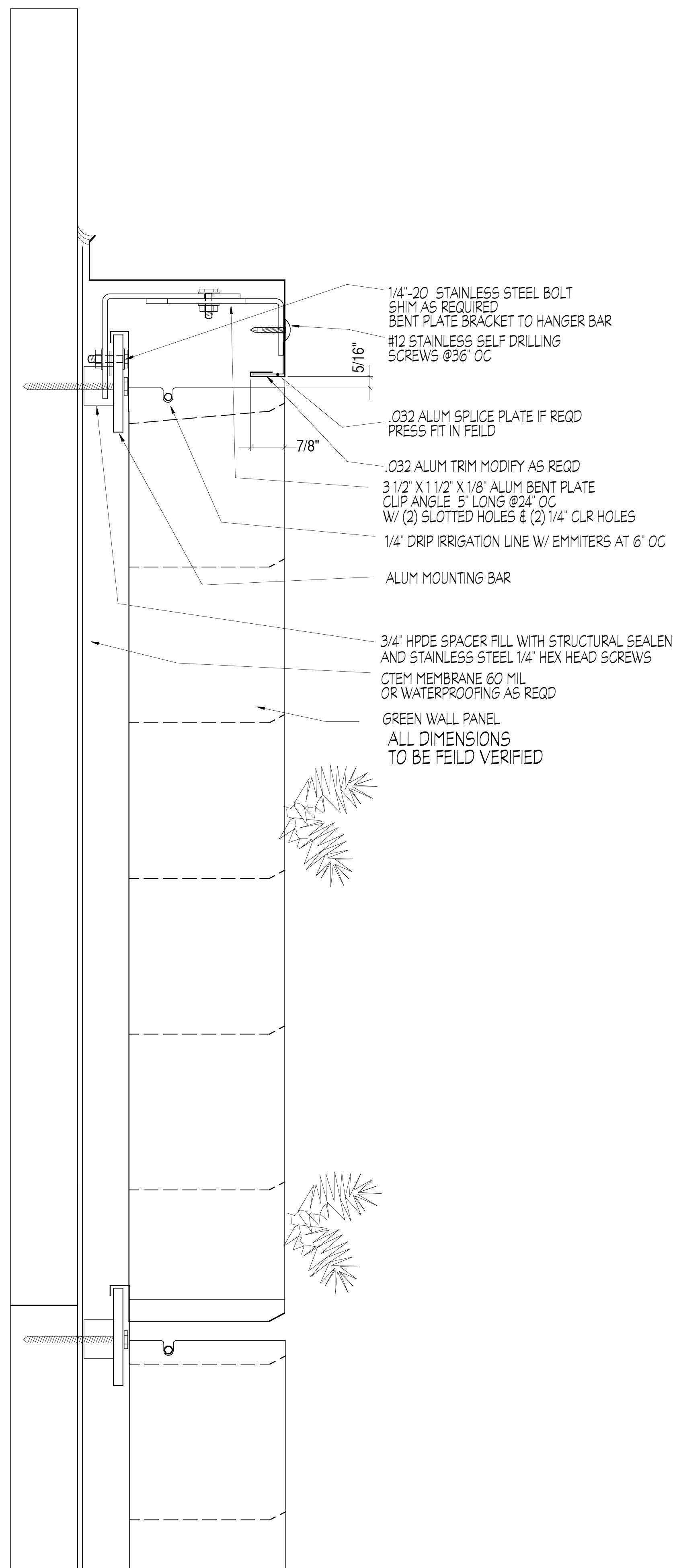
SECTION DETAIL GW PANEL
